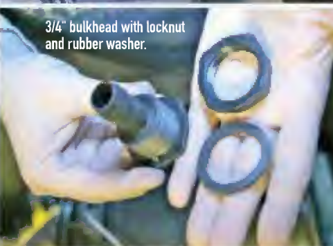
Screw the fittings into the bulkhead.
